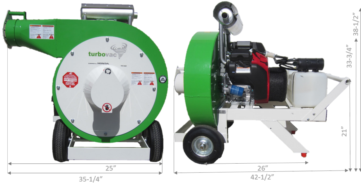
Part #TURBOVAC690SP-DD
